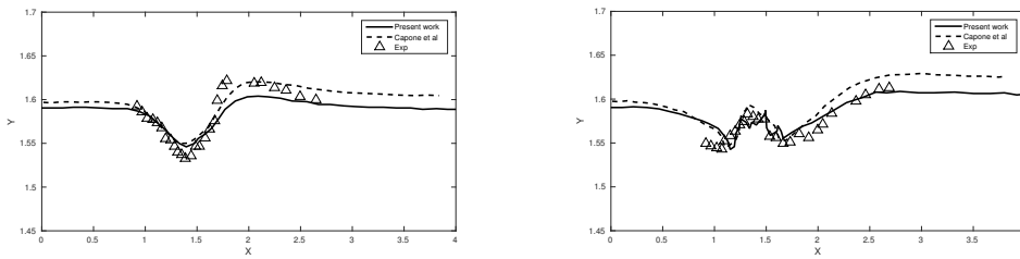
Figure 19: Submarine land-slide-generated water wave: Comparison between the free surfaces at t = 0.4[s] and t = 0.8[s] obtained with the proposed SPH model, the SPH model of Capone et al. [17] and the experimental results of Rzadkiewicz et al [66, 67].
