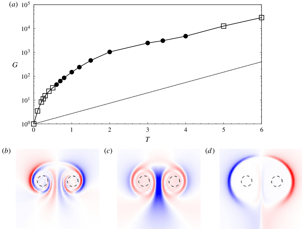
FIGURE 18. (Colour online) Results for Re = 1000 vortex pair: (a) variation of the linear optimal gain with horizon time. The gain obtained using the most unstable mode as the initial perturbation is indicated by a dotted line. The bottom row shows the velocity component parallel to the centreline for the LO-P corresponding to (b) T = 0.5 , (c) T = 1.0 and (d) T = 5.0 . The solid circles (respectively hollow squares) in (a) correspond to data points for which the LO-P is symmetric (respectively antisymmetric).
