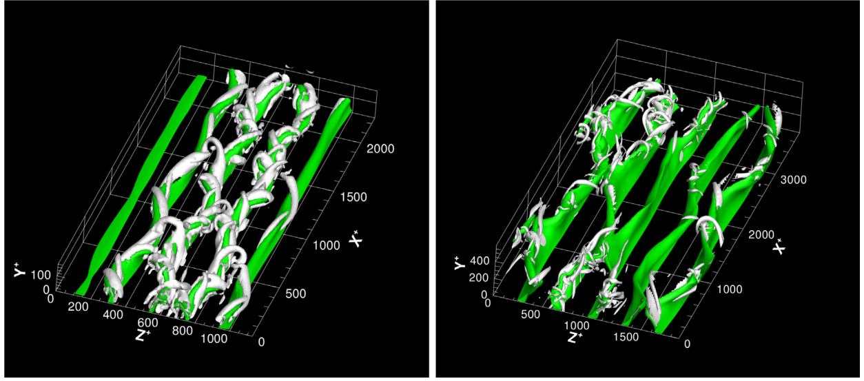
Fig. 3. Shape of the optimal perturbations at t = T : isosurfaces of negative streamwise velocity perturbation ( u'/u'_{\max} = 0.45 , green) and of the second invariant of the velocity gradient tensor, Q -criterion ( Q/Q_{\max} = 0.025 , grey). C180, E_0 = 10^{-2} (left) and C590, E_0 = 7.5 \times 10^{-4} (right). (For interpretation of the references to colour in this figure legend, the reader is referred to the web version of this article.)
