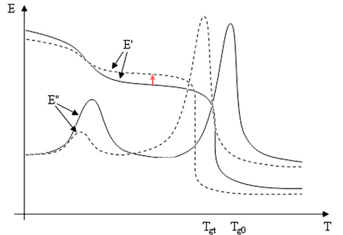
Fig. 1. Real ( E' ) and complex ( E'' ) part of the Young’s modulus of a virgin (solid line) and oxidized (dotted line) epoxy network sample. The arrow shows the increase of E' modulus in the glassy state.
