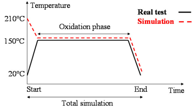
Fig. 7. Schematics of the loading history for numerical simulations following closely real test conditions.
