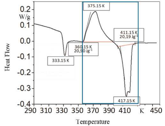
Fig. 1. DSC results of PLA
