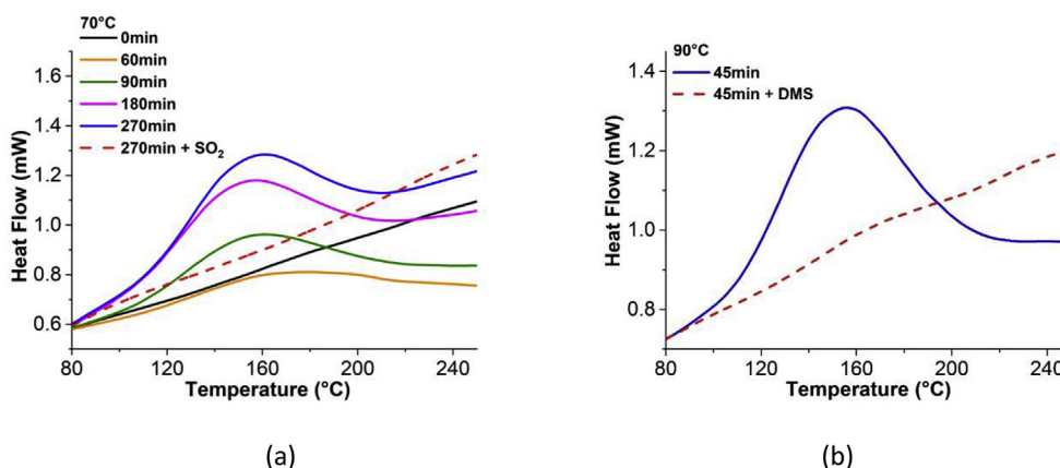
Fig. 1. DSC thermograms of M*-PDCPD exposed at 70 °C under air for various ageing times up to 270 min before (full line) and after (dashed line) SO 2 treatment (a), and exposed 45 min at 90 °C under air before (full line) and after (dashed line) DMS treatment (b).
