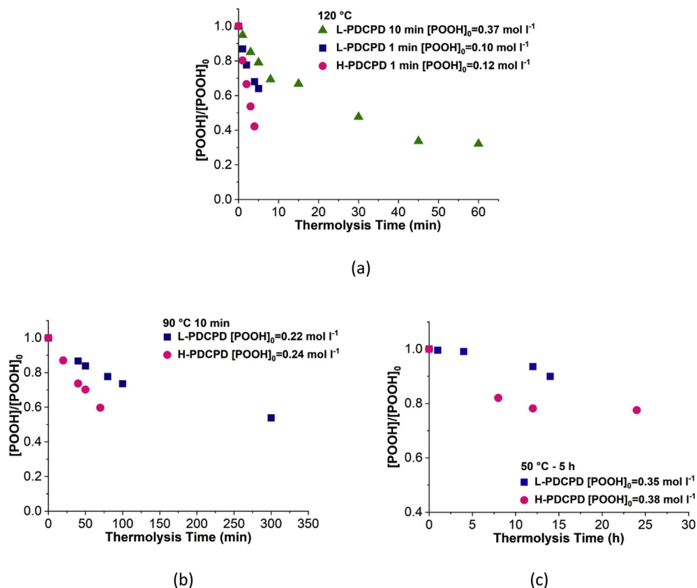
Fig. 8. Changes in hydroperoxides concentration for thermolysis of L-PDCPD ( \blacktriangle or \blacksquare ) and H-PDCPD ( \bullet ) at 120 (a), 90 (b) and 50 °C (c). NB: the caption indicates the temperature and time for ageing under air, and the corresponding POOH concentration after ageing and before thermolysis – see Fig. 6.
