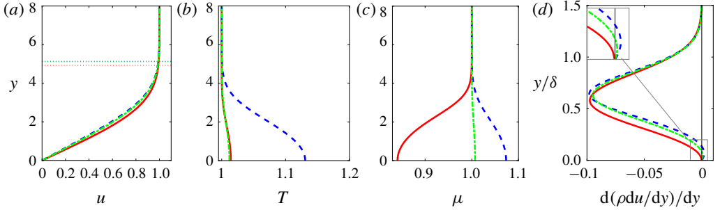
FIGURE 18. Influence of EOS model on similarity solutions for PP11 at M_\infty = 4.5 . Line legend as in table 4.
