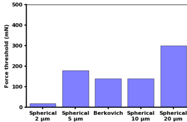
Figure 6: Force threshold versus the indenters where the scratch becomes visible.
