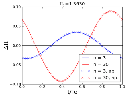
(c) cutting force variation over one oscillation period
