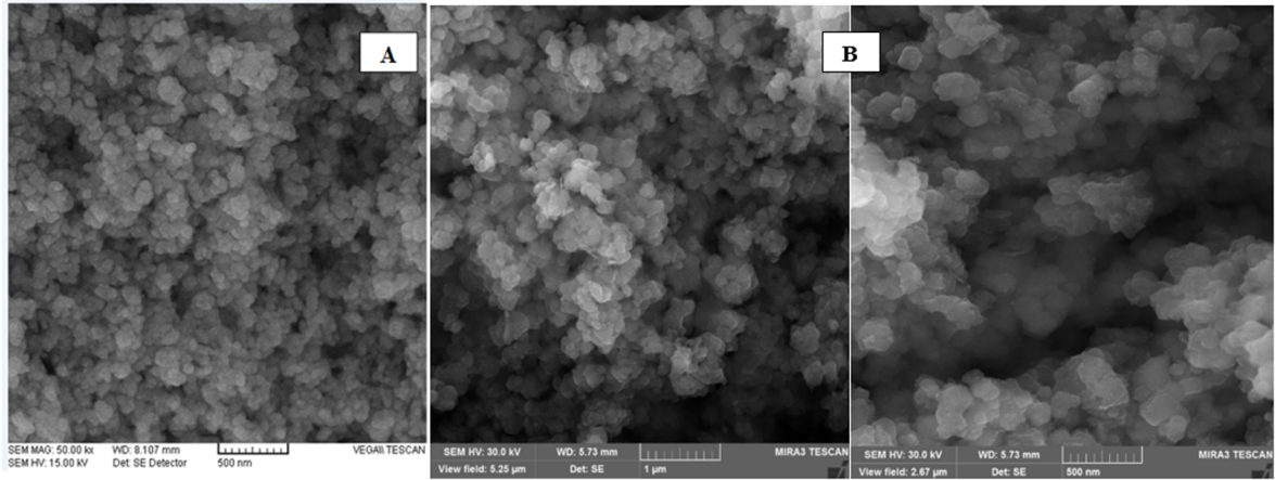
Fig. 4. SEM images of as-synthesized \text{CoFe}_2\text{O}_4 (A) and TCA (B) samples.
