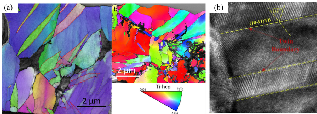
Fig. 11. (a) TKD image of twin boundaries in chips at cutting speed of 220 m/min conducted by Dargusch et al. (2018) and (b) the TEM image of twin boundaries in machined surface at cutting speed of 250 m/min conducted by Xu et al. (2019) during machining Ti6Al4V.
