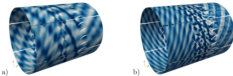
Fig. 13. Domain reconstruction 360° (FAN-OGV-swirl configuration); visualization of the pressure at time t = 10 ms for the two engine speeds: a) 41% Nm , b) 61% Nm . Cut radius r_c = 0.8 \cdot R .
