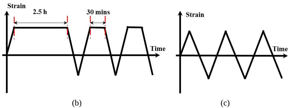
Fig. 3: (a) Dimensions of the investigated specimens (mm); (b) DWT loading pattern used for the CF experiments, and (c) SWT loading pattern used for the LCF experiments.
