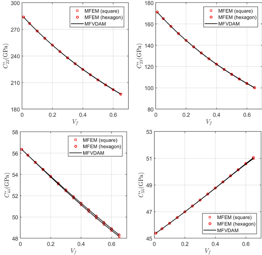
Fig. 5. Selected homogenized elastic moduli of a unidirectional BaTiO 3 /CoFe 2 O 4 composite as a function of BaTiO 3 volume content.
