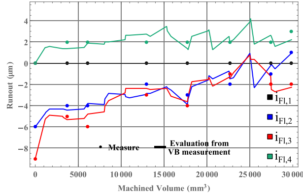
Fig. 17. Tool radial runout computed considering VB measurement and actual measured runout for AM material and a_e = 1 \text{ mm} .
