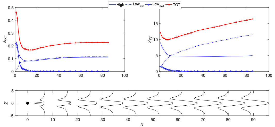
FIG. 26. Streamwise variation of the (left) amplitude of the streaks and of the (right) area associated with the streaks for the base flow.
