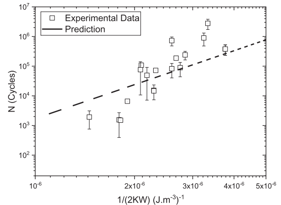
Fig. 9. Determination of b and B using unaged samples (A) and prediction of fatigue life as a function of the inverse of strain energy directly related to crosslink density (B) with R = 0.2 .
