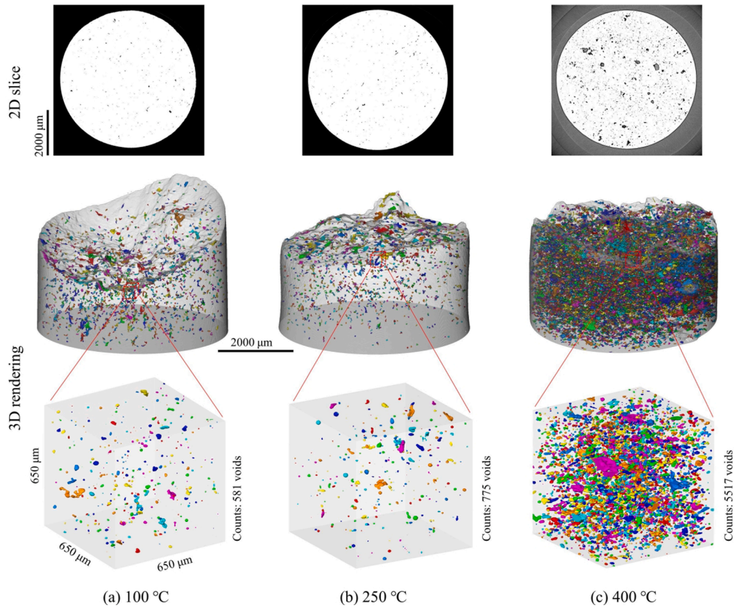
Fig. 10. 3D volume renderings of SR-μCT scans of ruptured specimens showing the distinct populations of microvoids between for samples tested at (a) 100 °C, (b) 250 °C and (c) the 400 °C. The false-colour coding is applied for clarity.
