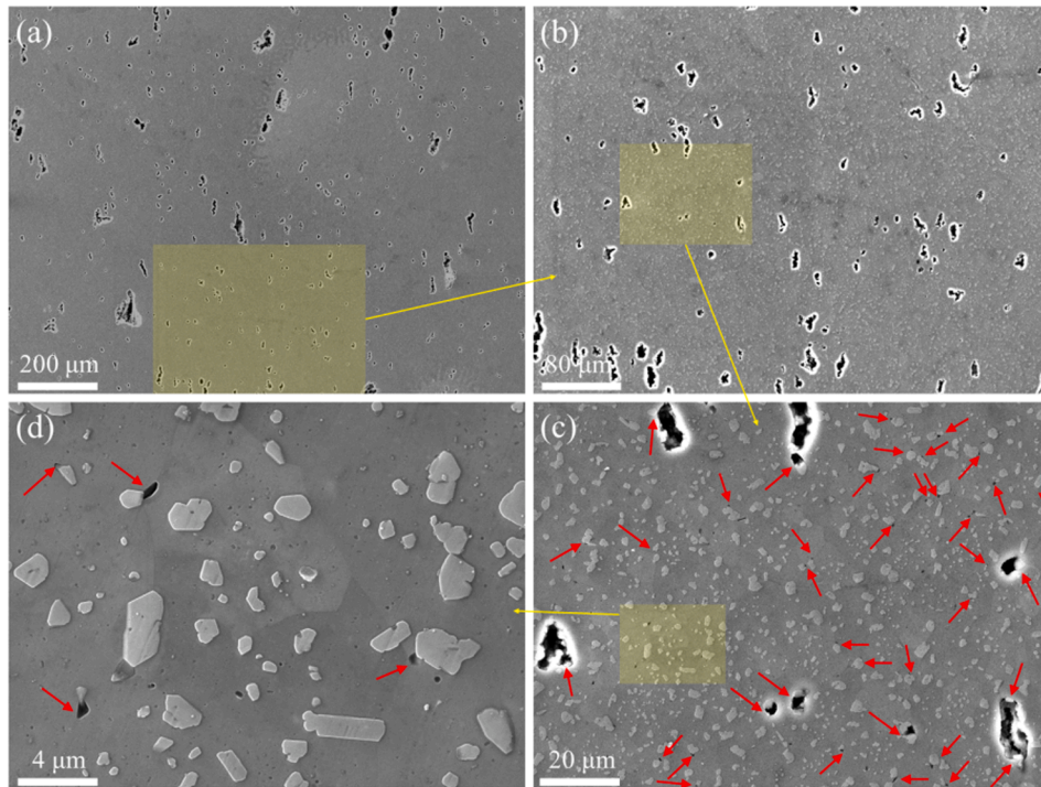
Fig. 11. Cross-sectional SEM images taken from a 400 °C SWT fatigued specimen with increasing magnification a) d) showing microvoids nucleating from Si precipitates, which are highlighted by red arrows. The imaged zones are located within ~ 2 mm away from the fracture surface.
