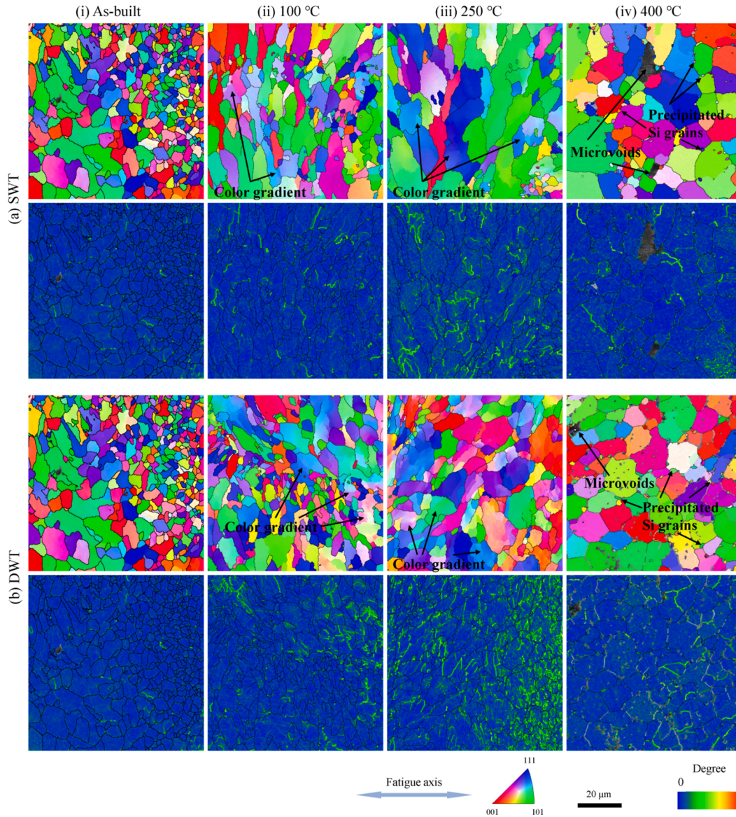
Fig. 7. Comparison of EBSD results between the as-built (with stress relieved) material and samples fatigued to failure for a) fatigued and dwell fatigue testes samples with the IPF maps (top) and KAM maps (bottom) where blue corresponds to low misorientation level, and red indicates the high misorientation levels. For the failed samples the areas studied were located within \sim 100 \mu\text{m} of the fracture surface.
