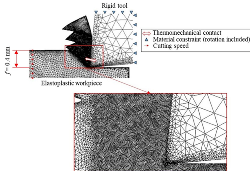
Figure 1. Example of the mesh for the orthogonal cutting case with special focus on the shear zone. f represents the feed or uncut chip thickness in orthogonal cutting.
