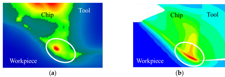
Figure 12. Experimental (a) and simulated (b) thermal fields during orthogonal cutting of Ti6Al4V. V_c = 7.5 m/min and f = 0.4 mm.
