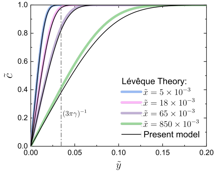
Figure 4: Comparison and validation of the model with L  v  que's theory. The vertical dashed line represents the validity limit of L  v  que's theory in case of \gamma = 3 .
