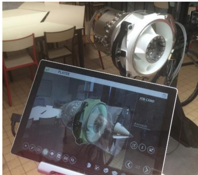
Figure 8. Representation of a complete aircraft engine, based on the support part.
