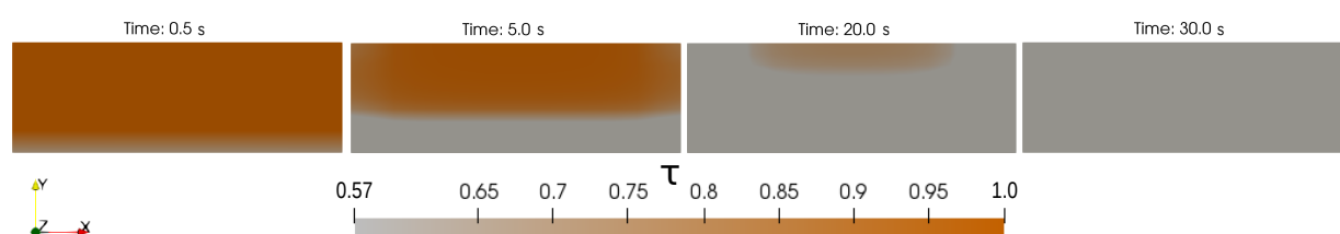
Figure 9. Advancement of pyrolysis of the wood log during the simulation. When \tau = 1 , no chemical reactions have still occurred. When \tau = 0 all the pyrolysis mechanisms have taken place and only char is left in the material. At time t = 0.5 s it can be seen how the pyrolysis process starts from the bottom of the material and at time t = 30 s how all the material has been pyrolysed.
