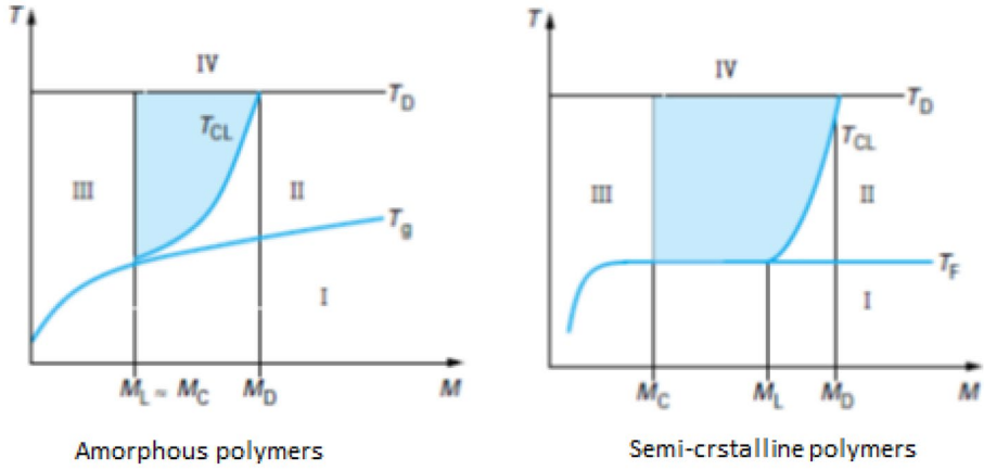
Fig. 2 Temperature-Molecular Weight diagram of thermoplastic polymers
