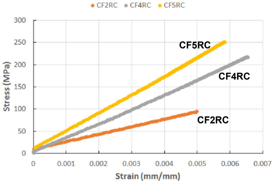
Fig. 42 Stress–strain of the printed specimens with CF with concentric fiber rings. The selected concentric rings of Carbon Fiber were 2, 4, and 5 [49]
