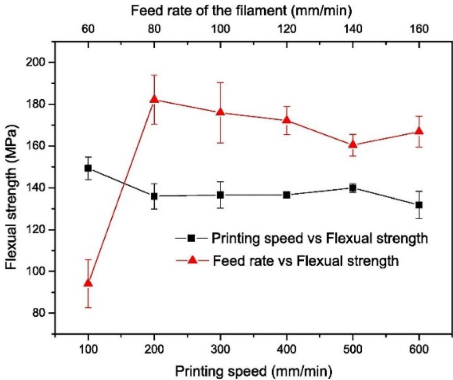
Fig. 24 Influence of feed rate of the filament and printing speed on the flexural strength of the 3D printed carbon fiber PLA composites [39]
