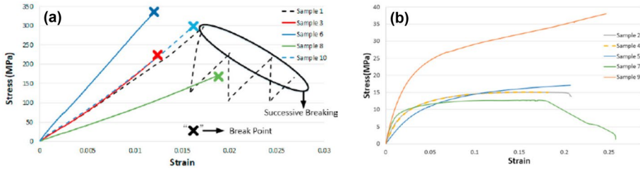
Fig. 35 Stress–strain curve and breaking points of 3D printed Kevlar fiber reinforced PLA composite with layups shown in Table 5 (a) samples 1, 3, 6, 8, 10 and (b) 2, 4, 5, 7, and 9 [45]
