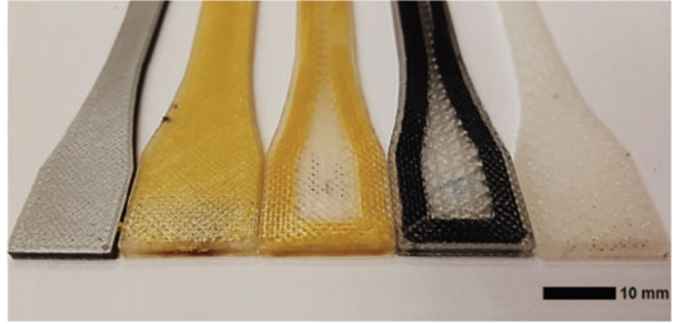
Fig. 30 3D-printed samples were used in the research. Left to right: PLA sample produced using Ultimaker 2 printer, \pm 45^\circ Kevlar fiber, unidirectional Kevlar fiber, unidirectional Kevlar fiber, and unreinforced nylon matrix [44]
