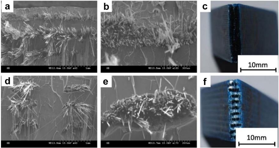
Fig. 23 Microstructures of the obtained fractured cross-section from the applied flexural test on the carbon fiber reinforced PLA composites with hatch spacing of 0.6 mm (a, b, c) and 1.6 mm (d, e, f), respectively: (a) and (d) overall cross-section, (b) and (e) interface, (c) and (f) fracture pattern [39]
