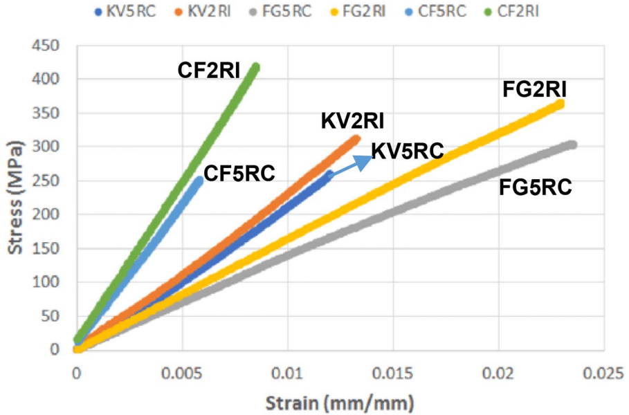
Fig. 44 Tensile Stress–strain curves related to tensile specimens using the two best-obtained fiber orientations [49]
