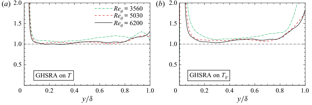
Figure 17. Classical GHSRA expressed in (3.13) (a) and GHSRA based on T_V , reported in (3.14) (b); ——— SRA estimation.
