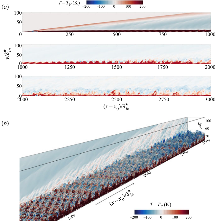
Figure 10. Instantaneous isocontours of T - T_V in a xy -plane and second invariant of the velocity gradient tensor, Q , coloured by T - T_V .
