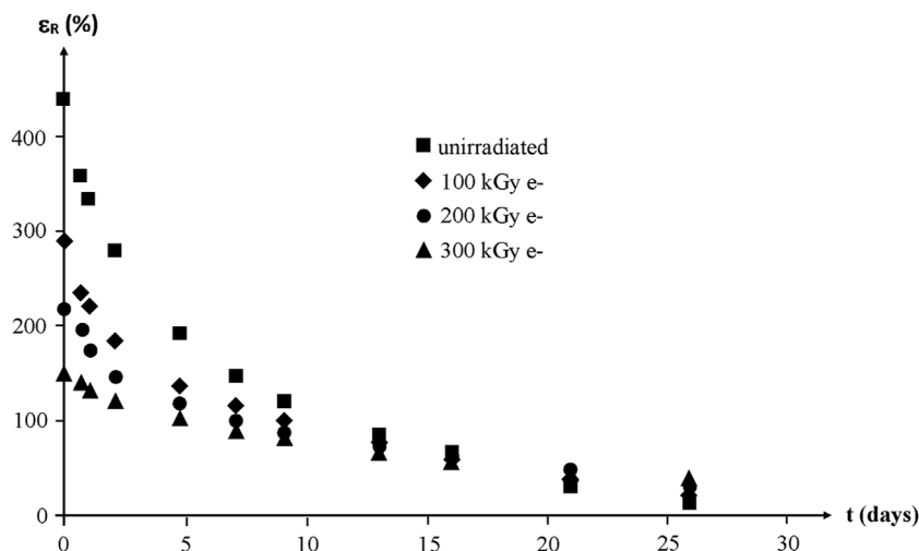
FIGURE 18 | Ultimate elongation of NBR samples with various radio-curing doses versus their time of exposure at 130°C in air. Results coming from the PhD dissertation of Lopitaux (2001).
