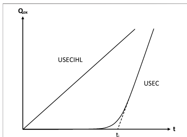
FIGURE 6 | Schematization of the general trend of the oxidation kinetic curves ( Q_{ox} = quantity of consumed oxygen) for the sets of assumptions indicated in this figure. Note that, in USEC, the assumptions relative to the constancy of initiation rate (I) and hydroperoxide stability (H) have been suppressed.
