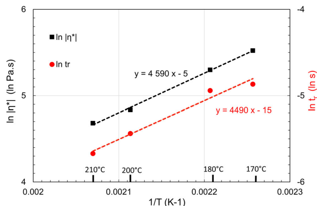
FIGURE 8 Arrhenius dependence of relaxation time and viscosity with temperature
