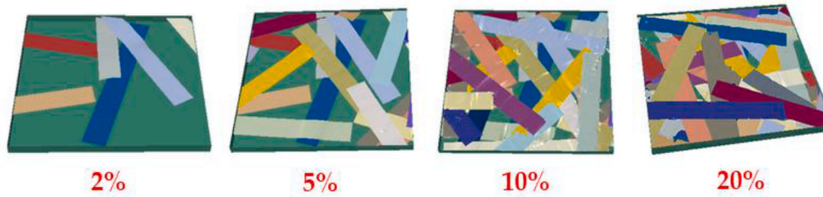
Fig. 15. Example RVE geometries ( 40 \times 40 \times 4.5 mm) for different volumes fractions.
