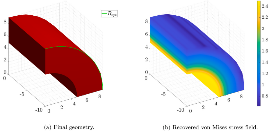
Fig. 10. Reference problem. Hybrid optimization result of the reference problem with the optimal analytic radius R_{opt}=9.0468 (a) and Von Mises stresses (b). The results were obtained using meshes of element size h_{TO} = 0.9563 and h_{SO} = 0.2391 .
