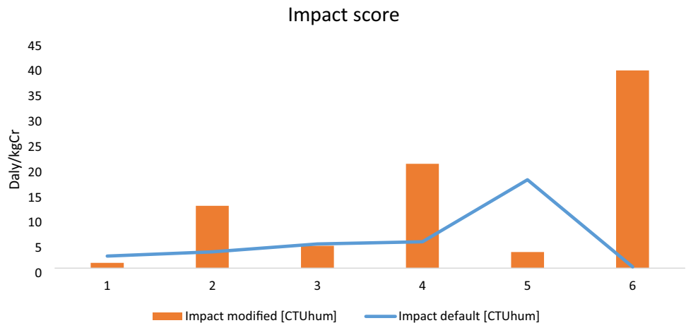
Fig. 9 The human health impact score modified and default of Cr in interfluvial areas, [Daly/kgCr], Lg scale. 1. Chulyum-Kiya; 2. Ob'-Chulyum-Kiya; 3. Chulyum-Ket'-Ulu-Yul; 4. Ob'-Chaya; 5. Ob'-Vasyugan-Chaya; 6. Chulyum-Ulu-Yul
