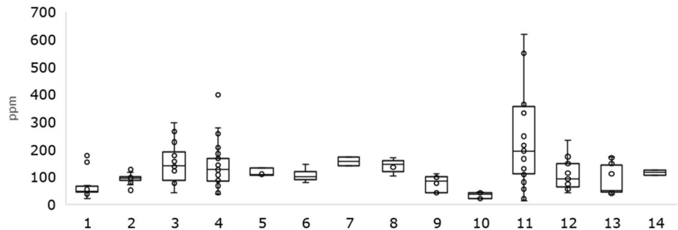
Fig. 7 The distribution of Cr in soils according to the administrative divisions of Tomsk oblast', [ppm]. Districts: 1. Asinovsky region, 2. Bakcharsky, 3. Verkhneketsky, 4. Zyryansky, 5. Kozhevnikovsky, 6. Kolpashovsky, 7. Krivosheinsky, 8. Molchanovsky, 9. Parabelsky, 10. Pervomaisky, 11. Teguldetsky, 12. Tomsky, 13. Chainsky, 14. Shegarsky
