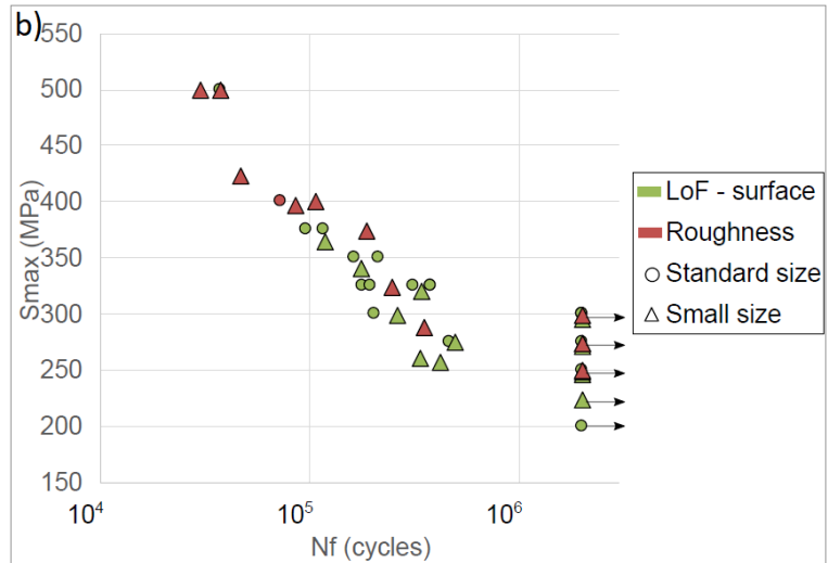
Figure 5: Correlation between the fatigue strength and the fatigue damage mechanisms for a) machined specimens and b) as-built specimens
