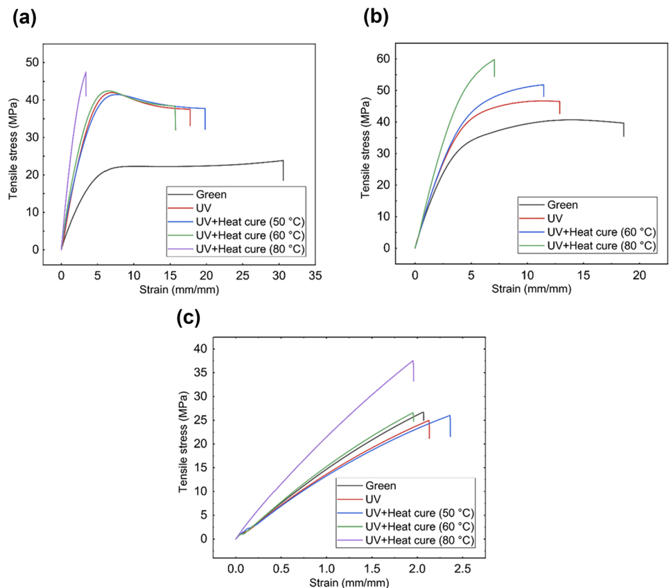
Fig. 6 Stress–strain curves with different post-curing conditions: a 0°-printed, b 45°-printed, and c 90°-printed
