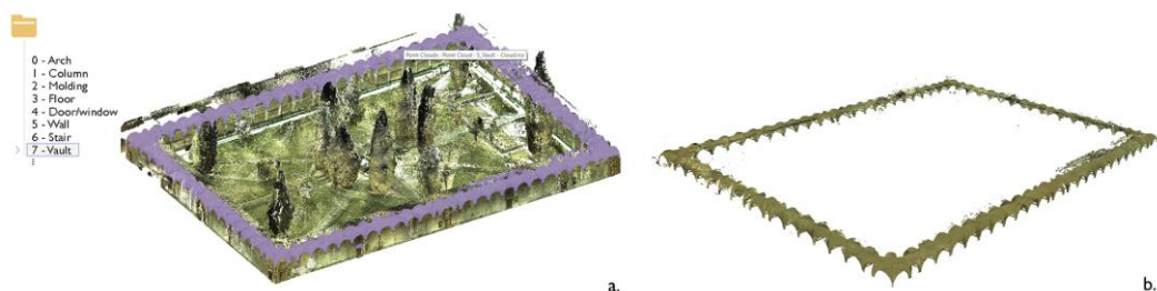
Figure 14. Segmented point cloud import. Selection (a) and isolation (b) of the 'Vault' class using example from the Grand cloister, Pisa Charterhouse.
