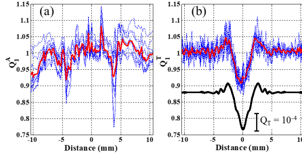
Figure 3 : Detection of ratio Q_I^A (a) and Q_I^T (b) from single shot detection (dot blue lines) and averaging of 10 detections (red continuous line). On (b), the signal presented in black (with its own amplitude scale) is obtained from linear simulations of a static inclusion.
