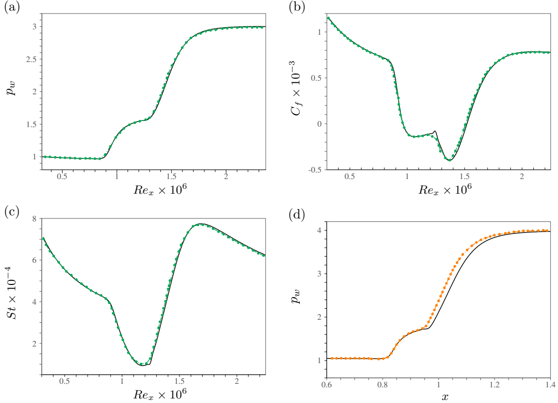
Figure 7: Verification test cases for the SWBLI configuration. Evolution of normalized wall pressure (a), skin friction coefficient (b) and Stanton number (c), compared with the reference solution of Sandham et al. [28]. Evolution of normalized wall pressure (d), compared with the reference solution of Volpiani [29].
