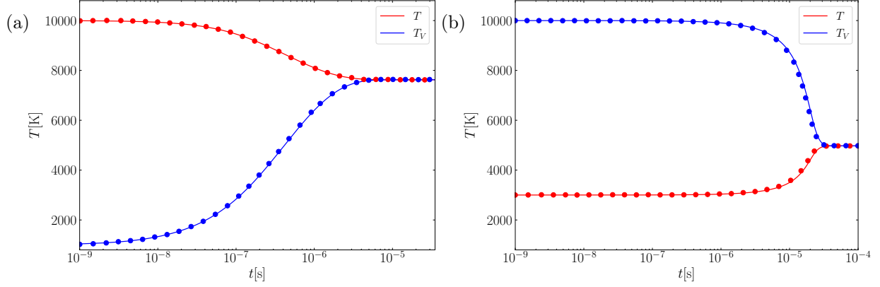
Figure 1: Translational-vibrational relaxation for vibrational heating (a) and vibrational cooling (b) of a N_2 heath bath; symbols from Casseau et al. [20].
