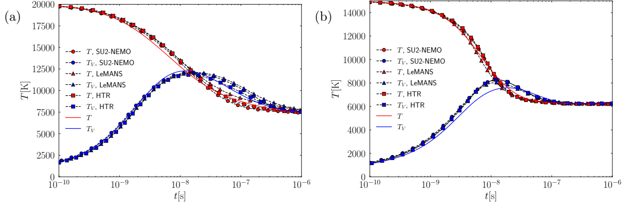
Figure 2: Dissociation/translational-vibrational relaxation heath bath for pure nitrogen (a) and air (b); symbols from Williams et al. [21].
