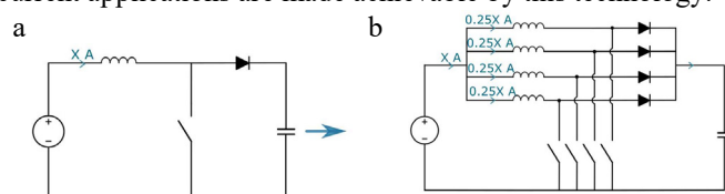
Fig. 3. Simple converter topology (a) and MIC topology (b).
