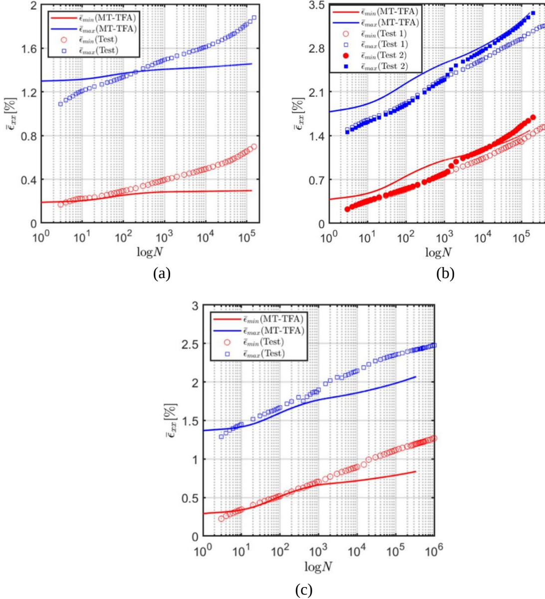
Fig. 6. Comparison of the maximum and minimum strains at each loading cycle for PA66/GF30 composites: (a) 0 deg under R=0.1 , \sigma_{max}=80\text{MPa} . (b) 45 deg under R=0.1 , \sigma_{max}=50\text{MPa} . (c) 90 deg under R=0.1 , \sigma_{max}=40\text{MPa} .
