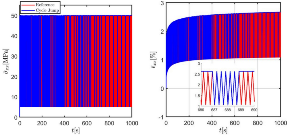
Fig. 5. Comparison of the differences in applied stress and the strain response between cycle jump simulation and cycle-by-cycle reference solution at 45^\circ loading configuration.
