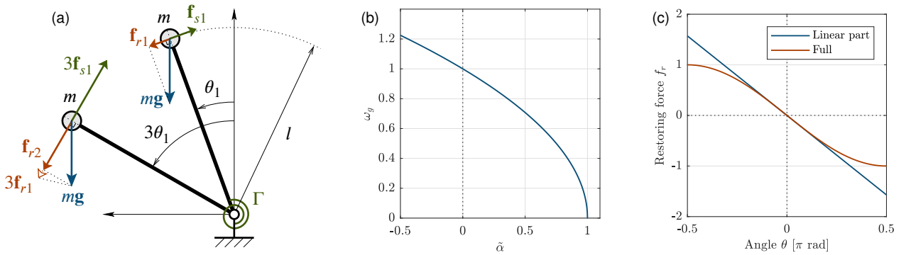
Figure 17: (a) Pendulum shown in two positions along with restoring force \mathbf{f}_r , (b) graph of the natural frequency \omega_g of the pendulum as a function of the gravity parameter \tilde{\alpha} (normalized), and (c) graph of the restoring force f_r as a function of angle \theta (normalized).
