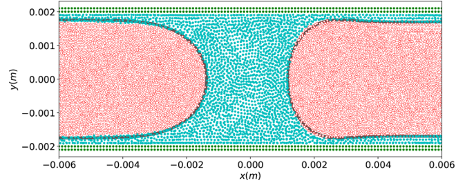
FIG. 4. Comparison of interface shape with the finite volume method result by Fujikoka et al. 30 Ca = 0.05 .
