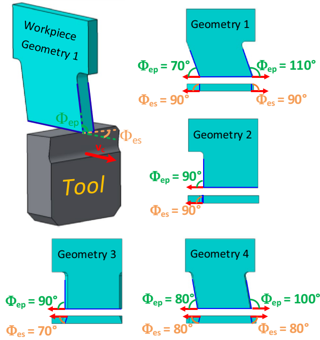
Fig. 5 Four sample designs leading to six different exit plane orientations: (\Phi_{ep} = 70^\circ, \Phi_{es} = 90^\circ) , (\Phi_{ep} = 80^\circ, \Phi_{es} = 80^\circ) , (\Phi_{ep} = 90^\circ, \Phi_{es} = 90^\circ) , (\Phi_{ep} = 90^\circ, \Phi_{es} = 70^\circ) , (\Phi_{ep} = 100^\circ, \Phi_{es} = 80^\circ) , (\Phi_{ep} = 110^\circ, \Phi_{es} = 90^\circ)
