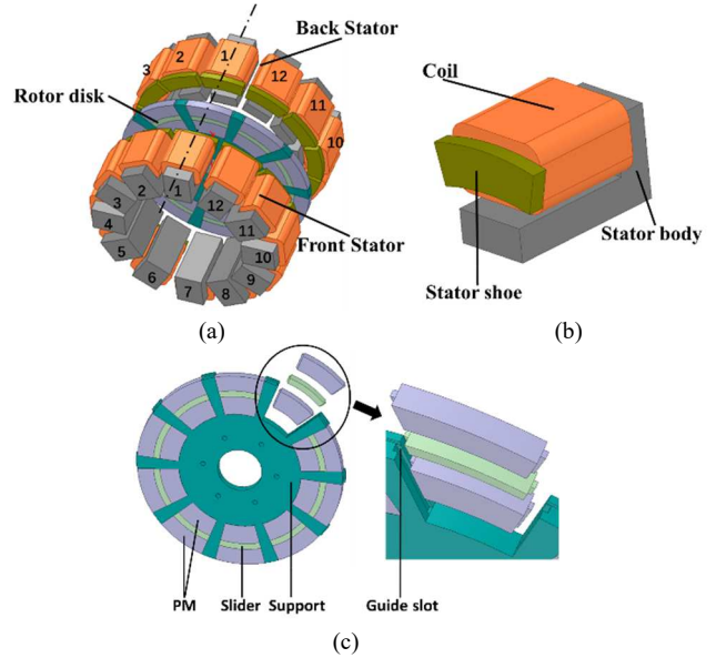
Fig. 2. Structure of previous 3-phase DTPAFM: (a) Total structure (b) Single armature stator core (c) Rotor part.
