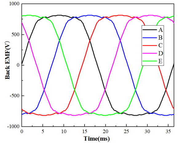
Fig. 8. The no-load back EMF waveform.
