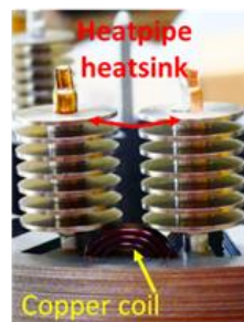
Figure 18: Condenser of the heat pipe over short end-winding coils
