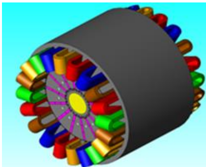
Figure 14: virtual view of prototype 1
