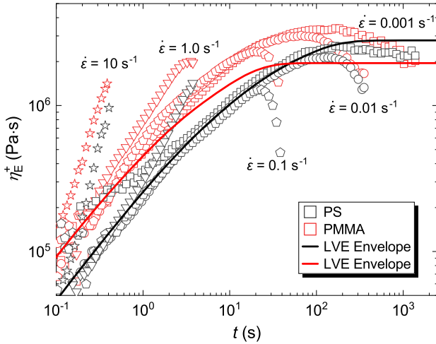
Figure 2: Extensional viscosity of PS and PMMA melts as a function of time, at 155 ^{\circ}\text{C} , at five chosen Hencky strain rates: 0.001, 0.01, 0.1, 1 and 10 \text{s}^{-1} . The solid lines represent the LVE envelope determined by Maxwell model.
