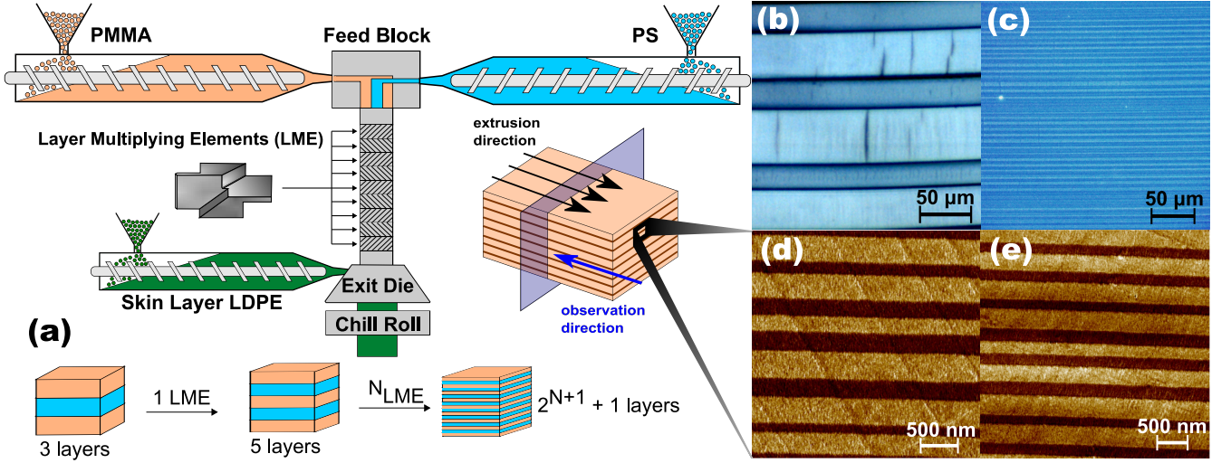
Figure 1: Multinanolayer coextrusion scheme (a) with typical images of fabricated films: (b) 17 layers (the black vertical strokes are compression lines present due to cutting); (c) 129 layers; (d) 2049 layers; (e) 4097 layers. On images from optical microscope (b, c), the lighter blue corresponds to PS, darker blue to PMMA. On AFM images (d, e), the colour gold represents PS layers while brown represents PMMA layers.
