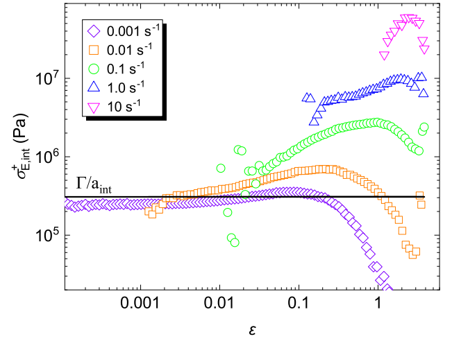
Figure 5: Measured interfacial stress as a function of strain for the same sample as in Figure 4.
