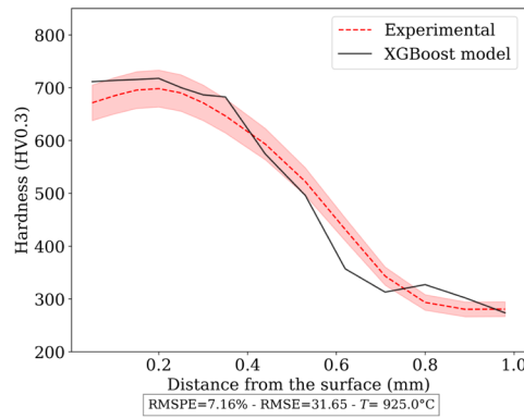
(c) Test Run # 14: tooth root
