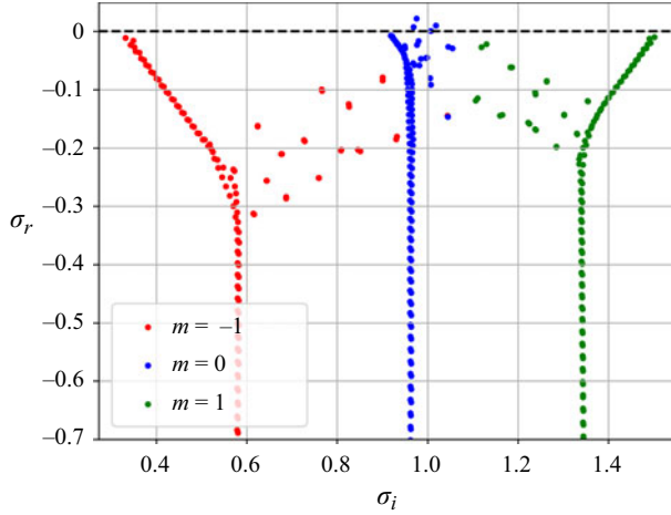
Figure 12. Secondary instability spectra for Re = 12\,000 , \beta_1 = -9.6 , A = 10^{-5} and \epsilon = 0.23 . Eigenvalues are coloured according to their respective Fourier mode. The values of the frequency and growth rate of the four most unstable modes are given in table 2 .
