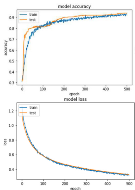
Figure 7: Performance of the MLP model after 500 epochs.
