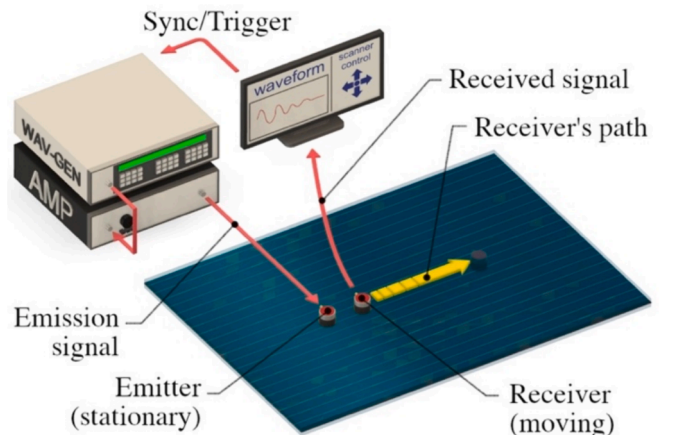
Fig. 3. Experiment to determine the distance between transducers for Lamb waves scan.
