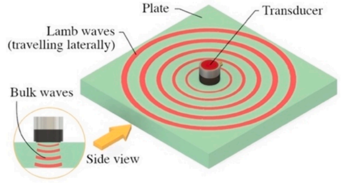
Fig. 1. Illustrations of the bulk waves traveling thickness-wise (used in conventional c-scan) and the Lamb waves traveling outwards from the excitation point, lateral to the plate's main plane.
