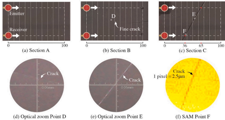
Fig. 6. (a, b, and c) The sections measured in the LW scan experiments to find damage indicators. (d and e) Optical microscope magnification of crack at the designated locations. (f) Scanning Acoustic Microscope (SAM) image of a typical crack.
