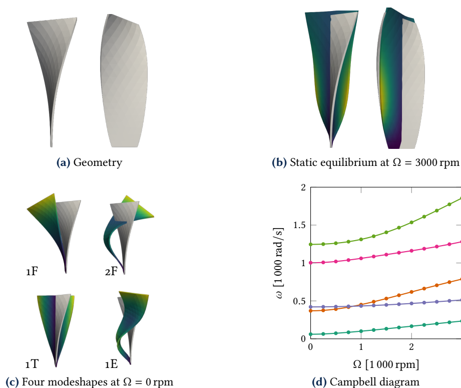
Figure 9 Linear characteristics of the twisted plate representative of a fan blade. In (b), static equilibrium position at \Omega = 3000 rpm (with colours) compared to the undeformed geometry (grey); amplitudes magnified by a factor 10 for readability. (d) colour code: [—] 1F; [—] 2F; [—] 1T; [—] 1E; [—] 3F.
