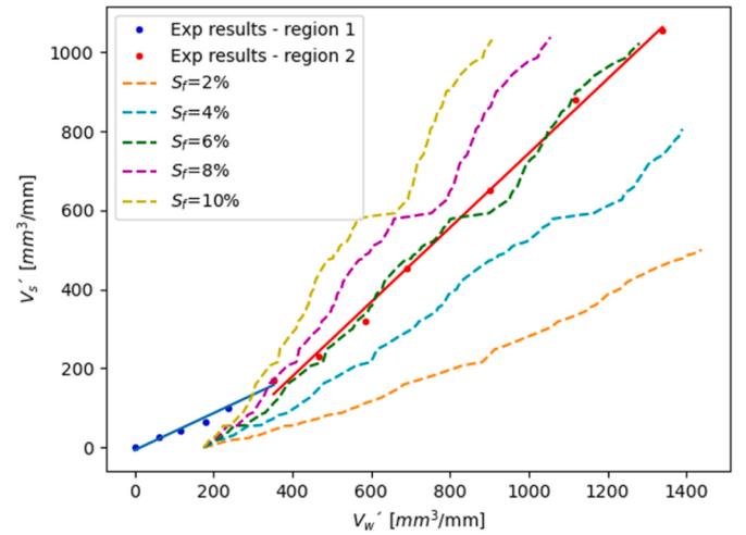
Fig. 21. Comparison of wear between multiscale simulations and experiments.
