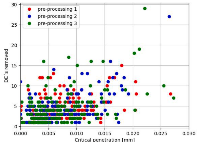
Fig. 16. Critical penetration vs DEs removed.
